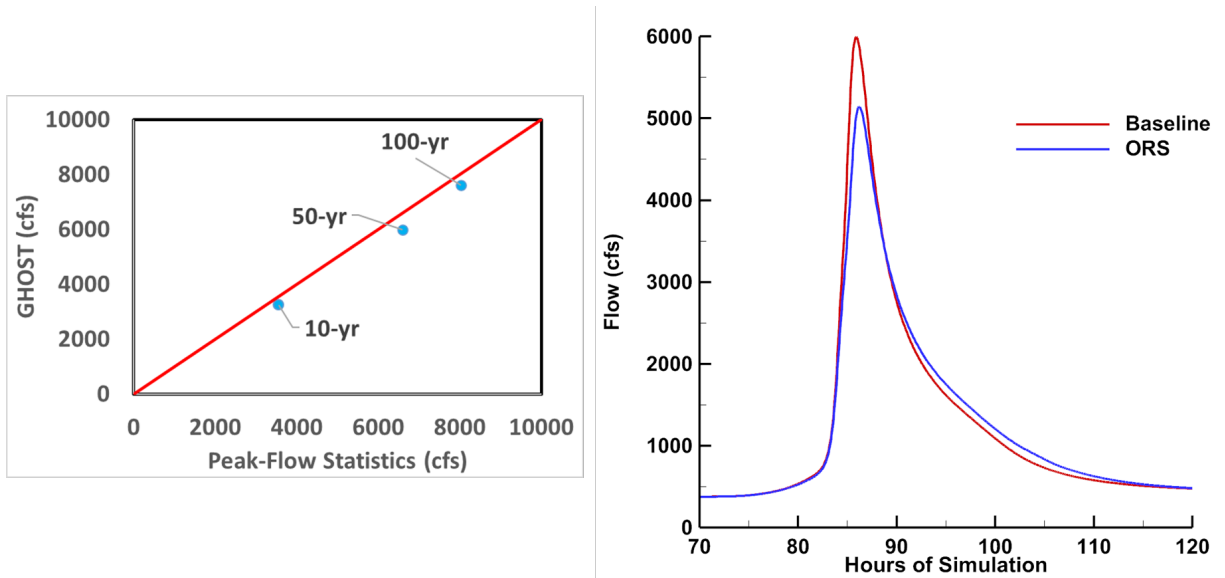
Figure 17. Left: Peak flow comparison at the watershed outlet, showing modeled values (vertical axis) versus estimates from regionalization and regression equations (StreamStats). Right: Hydrographs at the watershed outlet depicting model predictions for the 50-year storm with ORS and without ORS (Baseline) in place.
