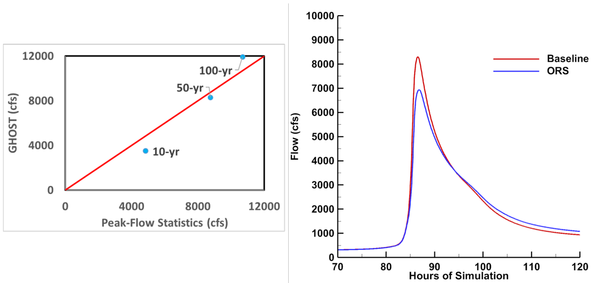
Figure 15. Left: Peak flow comparison at the watershed outlet, showing modeled values (vertical axis) versus estimates from regionalization and regression equations (StreamStats). Right: Hydrographs at the watershed outlet depicting model predictions for the 50-year storm with ORS and without ORS (Baseline) in place.
