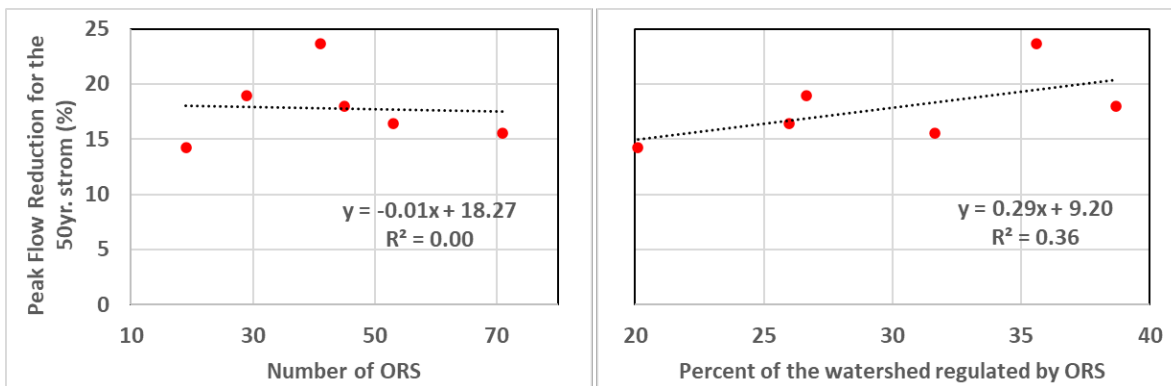
Figure 26. Left: Number of ORS vs. Peak flow reduction. Right: Percent of the watershed regulated vs. Peak flow reduction.
