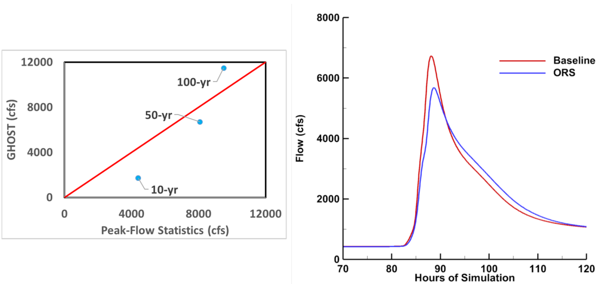
Figure 25. Left: Peak flow comparison at the watershed outlet, showing modeled values (vertical axis) versus estimates from regionalization and regression equations (StreamStats). Right: Hydrographs at the watershed outlet depicting model predictions for the 50-year storm with ORS and without ORS (Baseline) in place.
