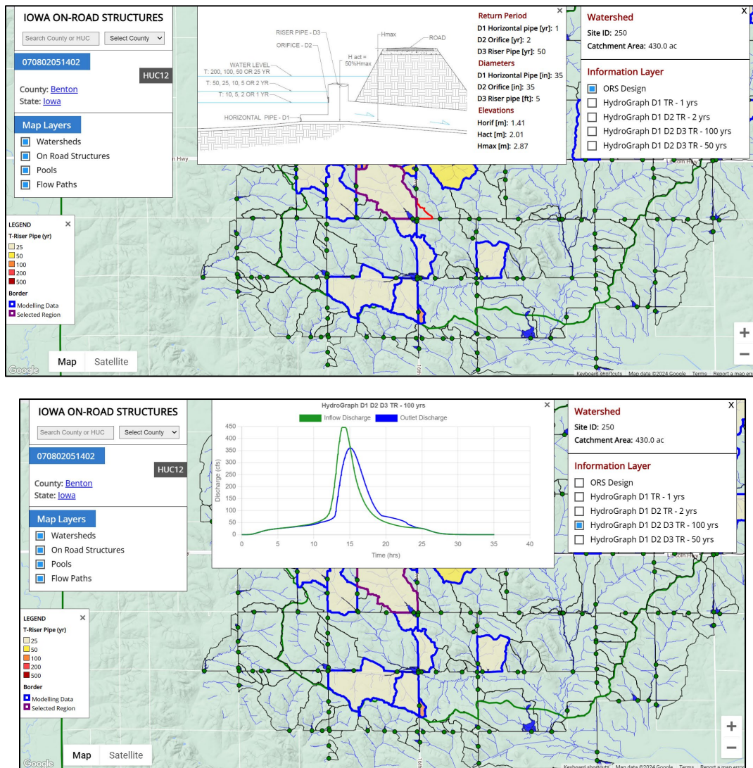
Figure 27 Top: Planning designs. Bottom: Inflow and outflow hydrographs for the 100-year storm. https://hydroinformatics.uiowa.edu/lab/idot-ors/
