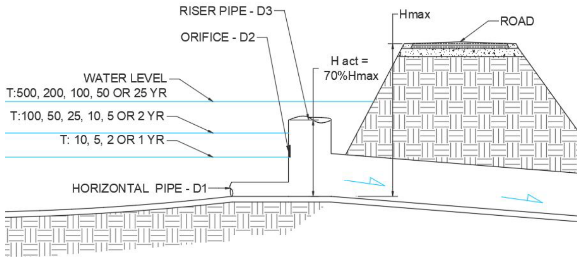
Figure 6. Typical ORS. The figure presents the three outlets (D1, D2, and D3), activation levels, and the different storms considered during the iterative design process.
