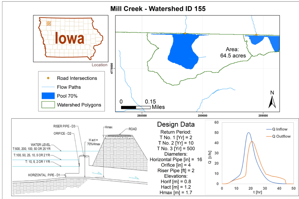
Figure 13. Planning designs. Example of the information generated by the scripts described in the methodology section.
