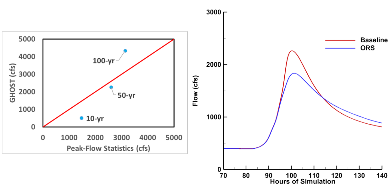
Figure 19. Left: Peak flow comparison at the watershed outlet, showing modeled values (vertical axis) versus estimates from regionalization and regression equations (StreamStats). Right: Hydrographs at the watershed outlet depicting model predictions for the 50-year storm with ORS and without ORS (Baseline) in place.
