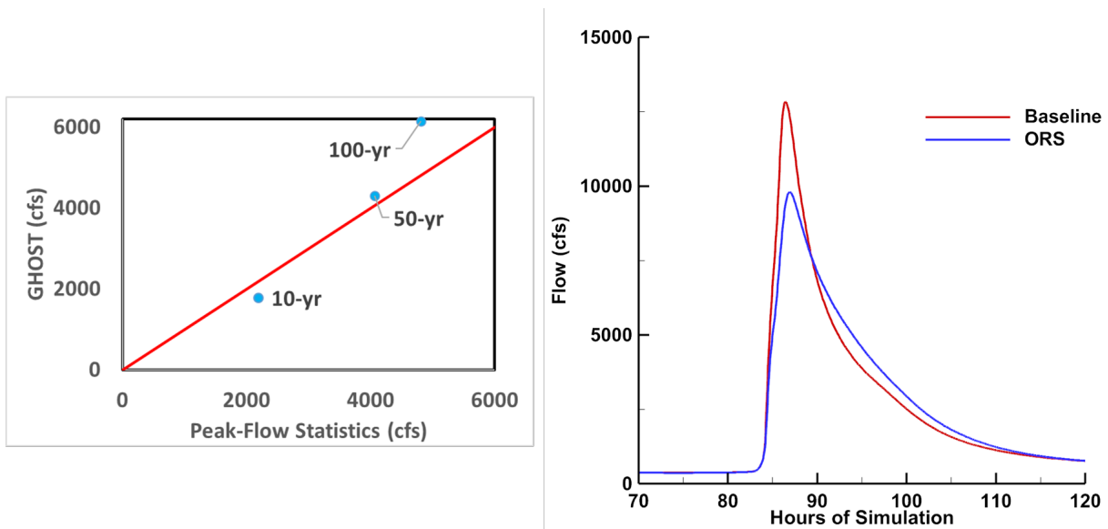
Figure 21. Left: Peak flow comparison at an interior point in the watershed, showing modeled values (vertical axis) versus estimates from regionalization and regression equations (StreamStats). Right: Hydrographs at the watershed outlet depicting model predictions for the 50-year storm with ORS and without ORS (Baseline) in place.
