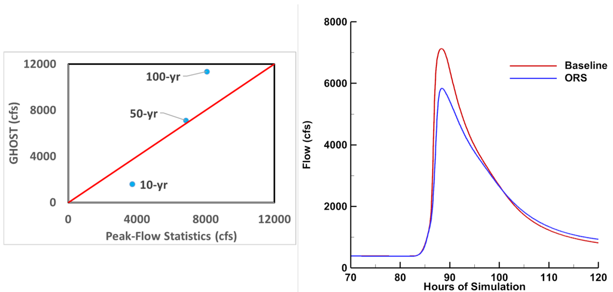
Figure 23. Left: Peak flow comparison at the watershed outlet, showing modeled values (vertical axis) versus estimates from regionalization and regression equations (StreamStats). Right: Hydrographs at the watershed outlet depicting model predictions for the 50-year storm with ORS and without ORS (Baseline) in place.
