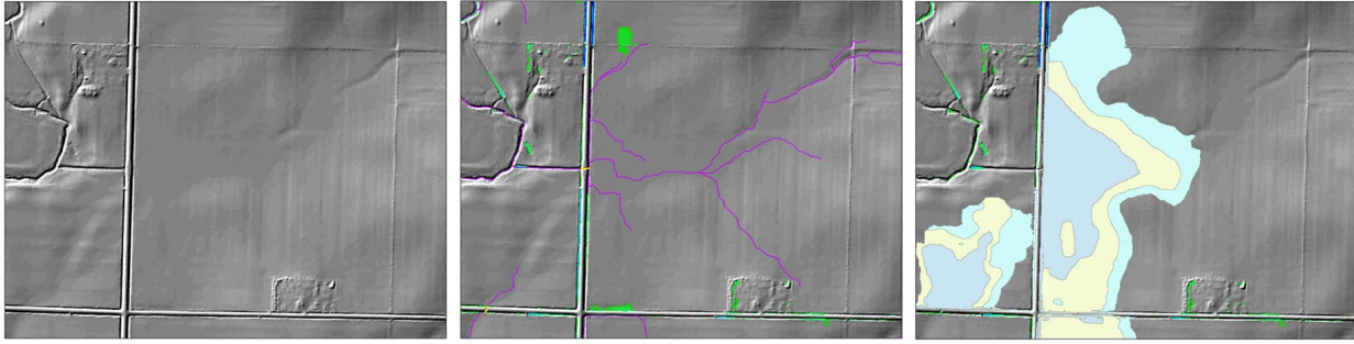
Figure 5. Left: DEM before hydroenforcement. Middle: cuts (culverts) were added, and flow paths were generated. Right: storage pools were estimated assuming three different ORS elevations: 50%, 70%, and 90% of the road height.
