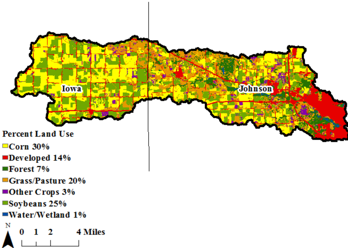
Figure 2.8. Land use composition in the Clear Creek Watershed, per the 2017 USDA Cropland Data Layer.
