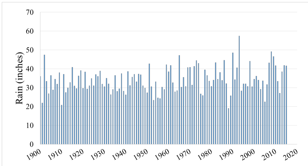
Figure 2.3. Bar graph of annual precipitation.
