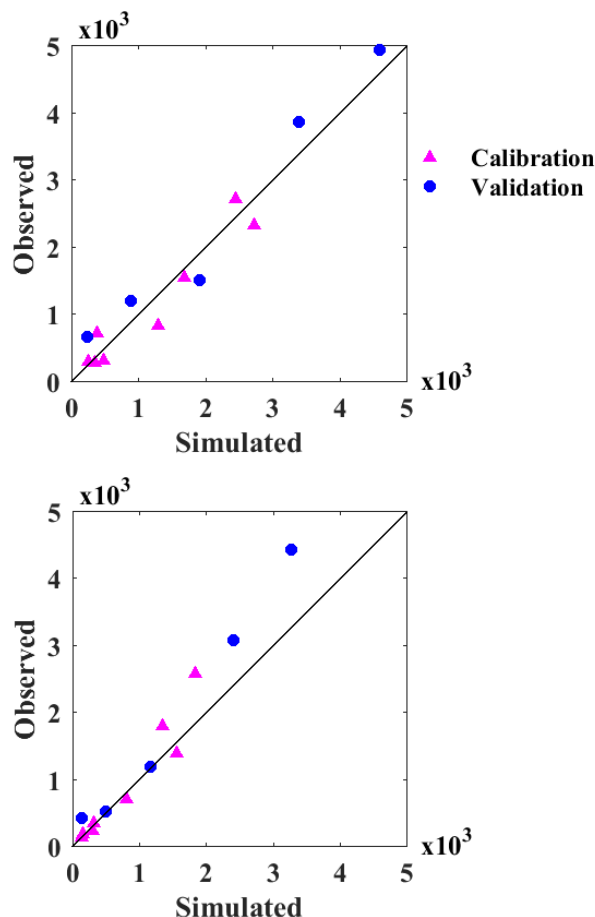
Figure 3.7. Simulated versus observed annual maximum peak daily discharges (cfs) for Clear Creek at Coralville (top) and Oxford (bottom). Results are shown for both the calibration (2002-2010) and validation (2011-2016) periods.
