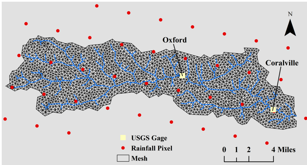
Figure 3.3. Computational mesh and rainfall pixels.
