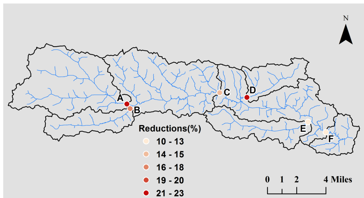
Figure 4.11. Average peak discharge reduction (%) for index points in the Clear Creek Watershed. Baseline vs. Distributed Storage (historic precipitation).
