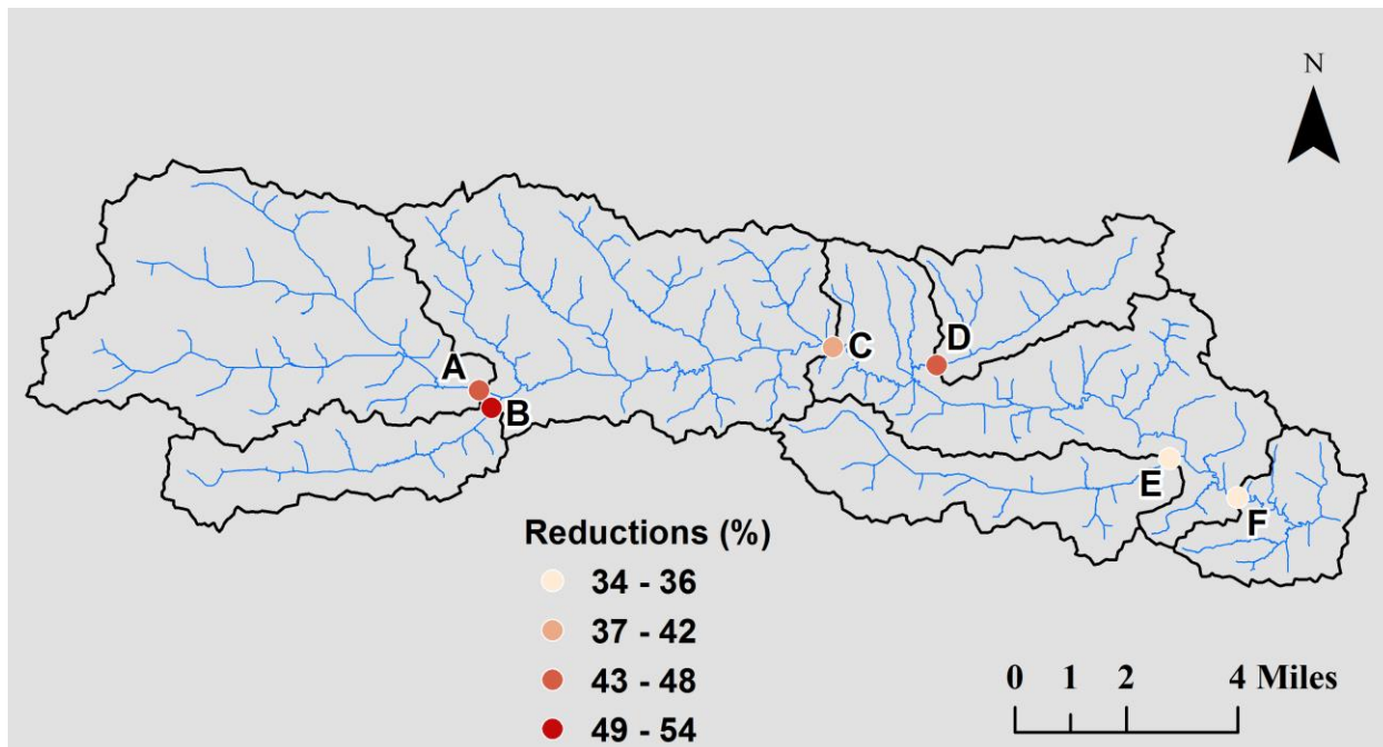
Figure 4.7. Average peak discharge reduction (%) for index points in the Clear Creek Watershed. Baseline vs. Cover Crop/No-Till (historic precipitation).
