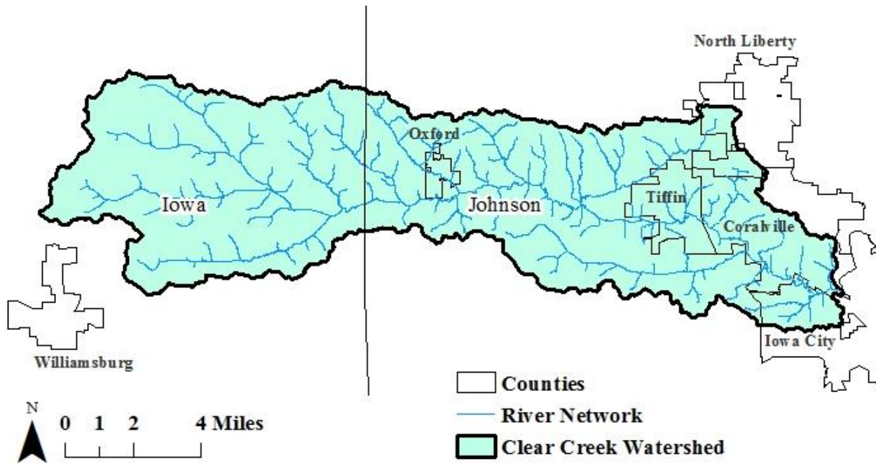
Figure 2.1. The Clear Creek Watershed (HUC10 0708020904), drains 104 mi 2 . The Clear Creek River joins the Iowa River in Coralville, IA.
