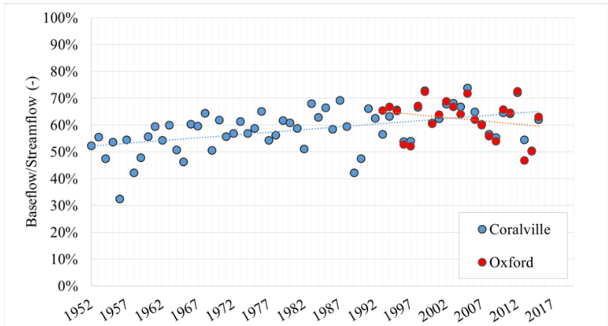
Figure 2.5. Annual ratio of baseflow to streamflow.
