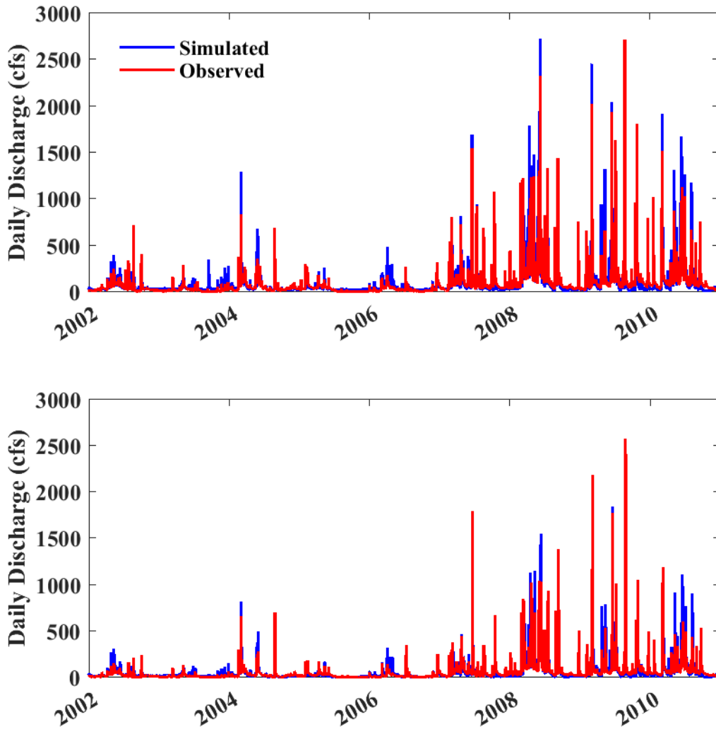
Figure 3.4. Observed and simulated daily flow time series. Calibration period. Top: Coralville, Bottom: Oxford. Measured flows were obtained from USGS gauge stations. Near Coralville: USGS 05454300, near Oxford: USGS 05454220.
