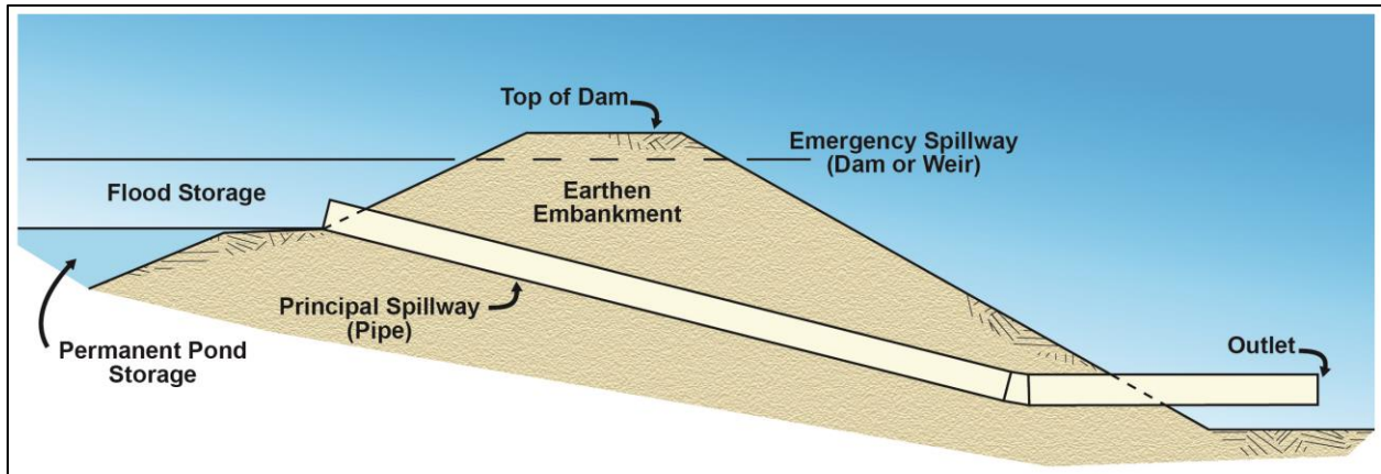
Figure 4.8. Schematic of a pond constructed to provide flood storage.
