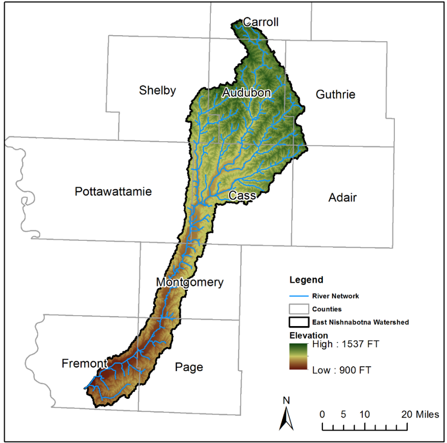
Figure 2.6. Topography of the East Nishnabotna River Watershed.
