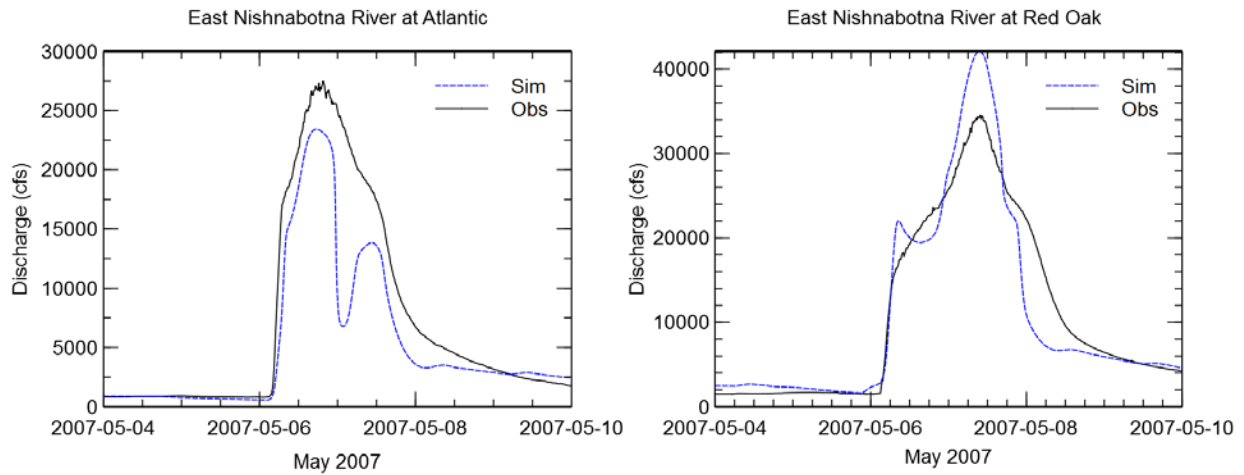
Figure B.6. Validation Storm Events – May 4–10, 2007
