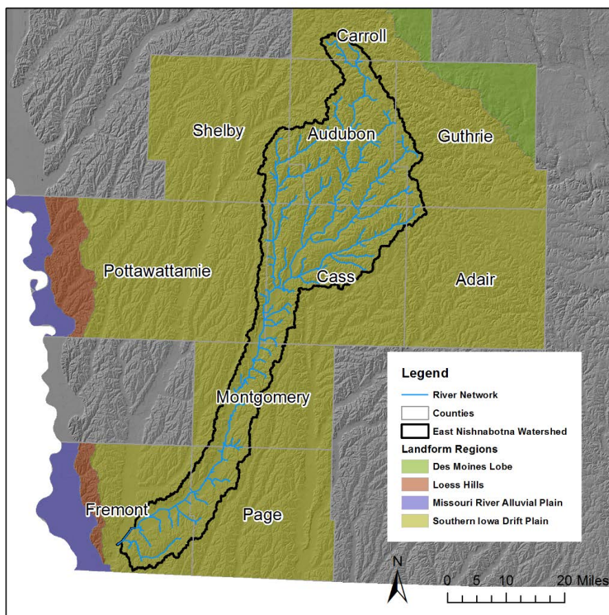
Figure 2.2. Defined Landform Regions of the East Nishnabotna River Watershed.
