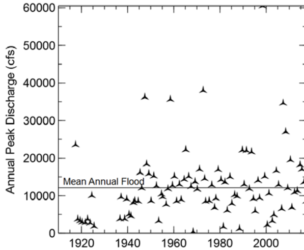
Figure 2.13. Annual maximum peak discharges observed at the Red Oak USGS stream gauge station.
