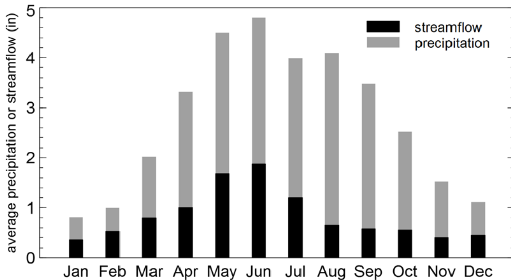
Figure 2.12. Monthly water cycle for the East Nishnabotna River Watershed. The plots show the average monthly precipitation (inches) and the average monthly streamflow (inches). The average monthly estimates for precipitation and streamflow are based on the period 1950–2017.
