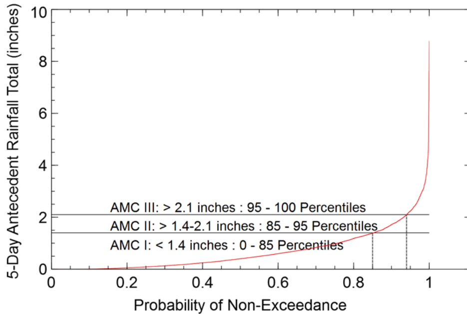
Figure B.1. Five-day rainfall total cumulative distribution function (CDF) for the East Nishnabotna River Watershed. We computed the CDF using the daily basin average precipitation computed between May and September of each year over a 68-year period (1950–2017).
