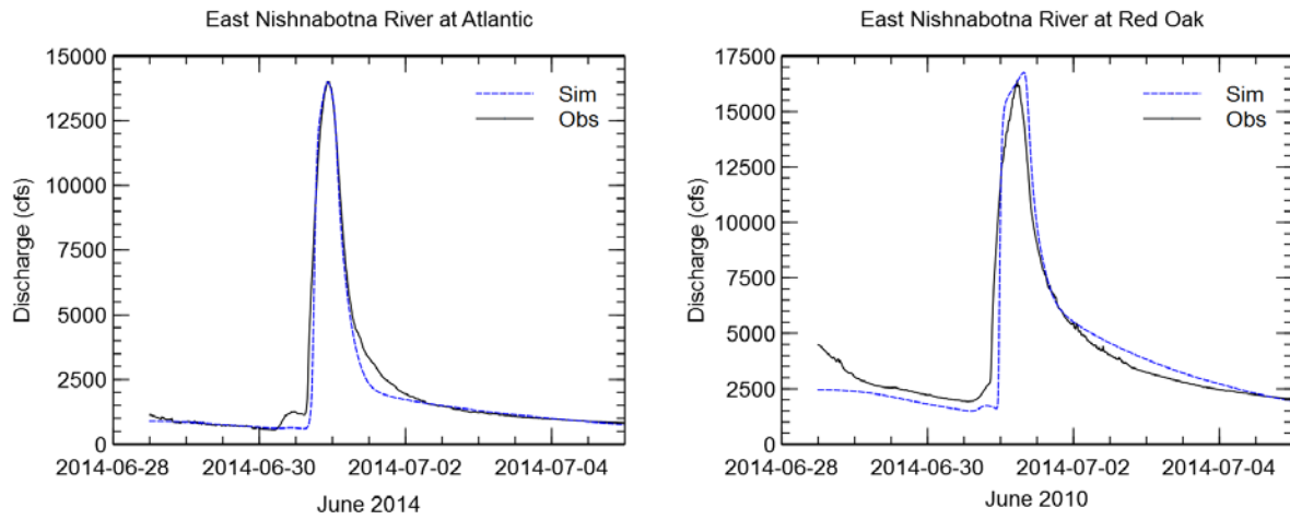
Figure B.10. Validation Storm Events – June 28–July 04, 2014
