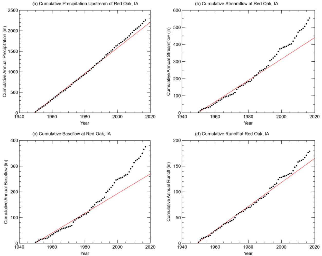
Figure 2.10. Cumulative annual totals for: (a) precipitation; (b) streamflow; (c) baseflow; and (d) runoff at Red Oak, Iowa.
