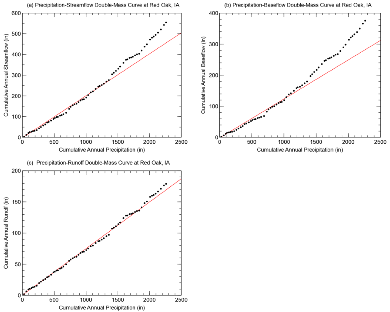
Figure 2.11. Double-mass curves using cumulative annual precipitation with cumulative annual (a) streamflow, (b) baseflow, and (c) runoff at Red Oak, Iowa.
