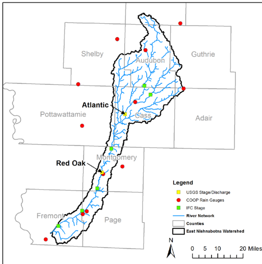
Figure 2.8. Hydrologic and meteorologic instrumentation in the East Nishnabotna River Watershed. Stage/discharge gauges (8) are shown in yellow or green, while NOAA-partnered daily- or sub-hourly measuring precipitation gauges (13) are shown in red.
