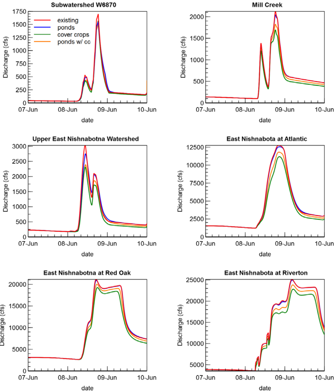
Figure 4.18. Hydrograph comparisons – with ACPF ponds, with 100% use of cover crops, and a combination of ACPF ponds and 50% use of cover crops for the June 2008 event.
