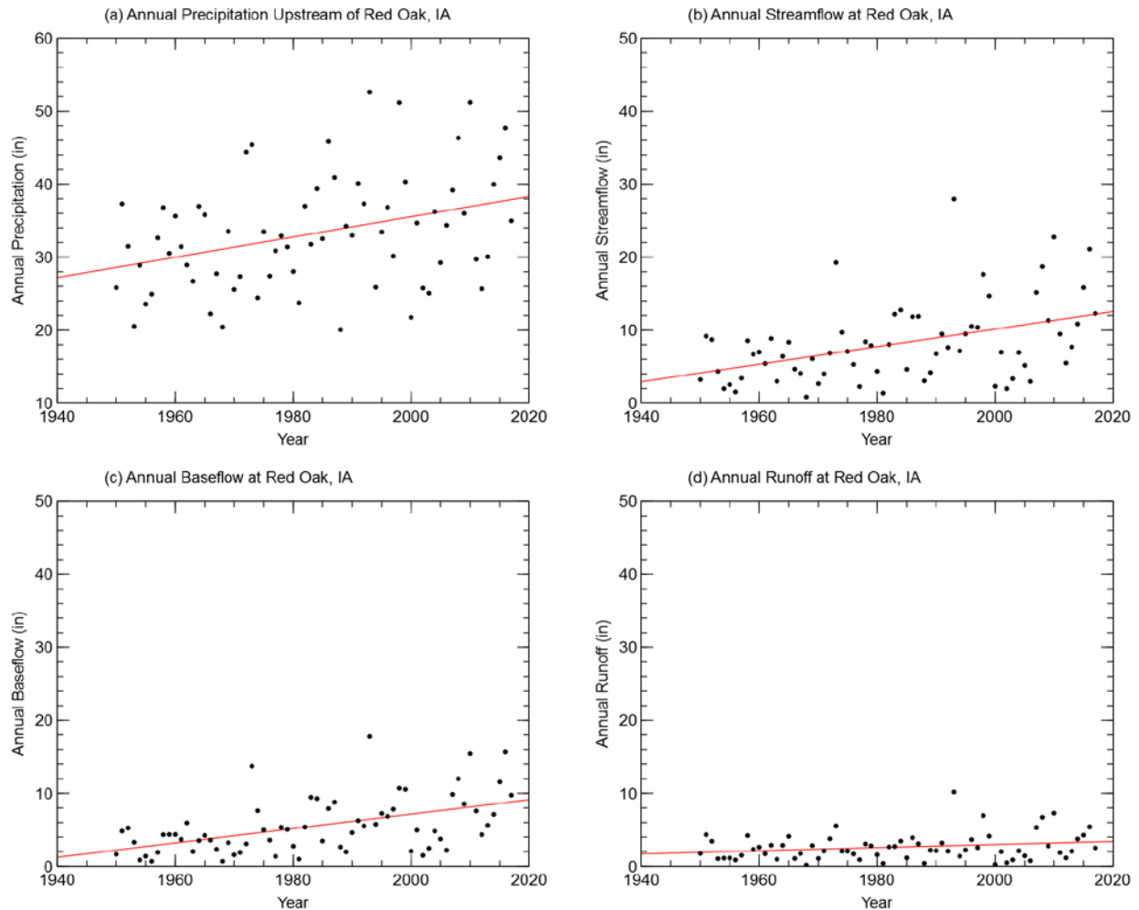
Figure 2.9. Annual totals for: (a) precipitation; (b) streamflow; (c) baseflow; and (d) runoff at Red Oak, Iowa.
