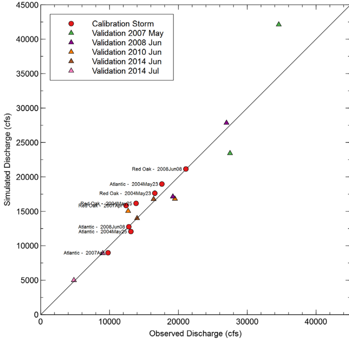
Figure B11. Comparison of simulated and observed peak discharges at USGS stage/discharge gauge locations in the East Nishnabotna River Watershed for calibration and validation events.
