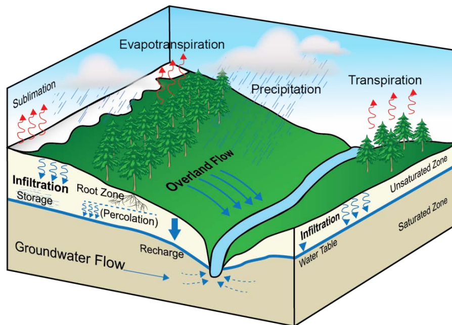
Figure 3.1. Hydrologic processes that occur in a watershed. Phase I modeling only considered the precipitation, infiltration, and overland components of the water cycle.
