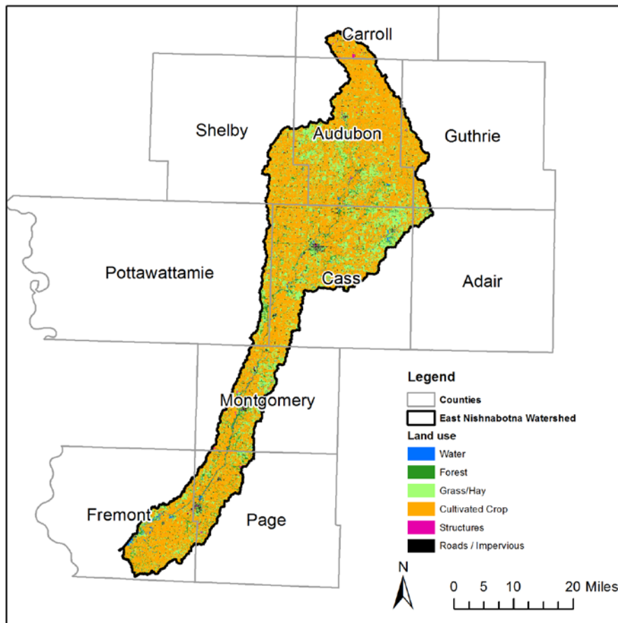
Figure 2.8. Land use composition in the East Nishnabotna River Watershed, according to the 2009 HRLC dataset provided by Iowa DNR.
