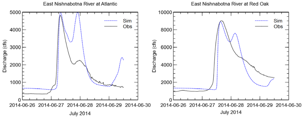
Figure B.9. Validation Storm Events – June 26–30, 2014
