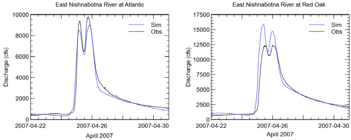
Figure B.4. Calibration Storm Events – April 22–30, 2007
