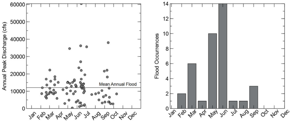
Figure 2.14. Annual maximum peak discharge and the calendar day of occurrence at Red Oak, Iowa (left), and the flood occurrence frequency by month (right).
