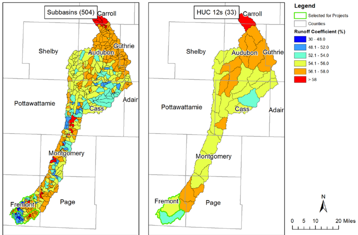
Figure 4.2. Runoff potential in the East Nishnabotna River Watershed. Runoff coefficients computed for each subbasin (left) and HUC 12 watershed (right) for a 6-inch, 24-hour design storm are shown. Higher runoff coefficients appear in red.
