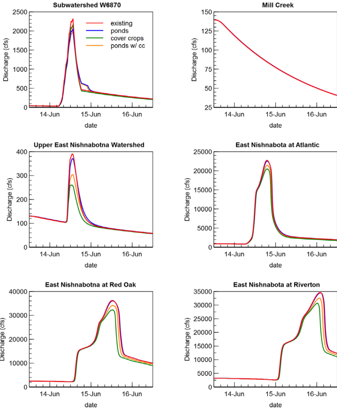
Figure 4.26. Hydrograph comparisons – with ACPF ponds, with 100% utilization of cover crops, and a combination of ACPF ponds and 50% utilization of cover crops for the translated Ames, Iowa, June 2018 event.
