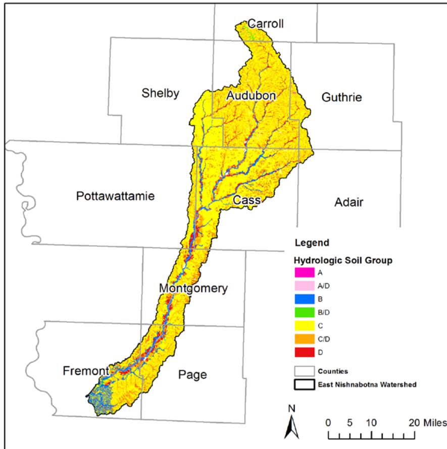
Figure 2.5. Distribution of hydrologic soil groups in the East Nishnabotna River Watershed. Hydrologic soil groups reflect the degree of runoff potential a particular soil has, with Type A representing the lowest runoff potential and Type D representing the highest runoff potential.
