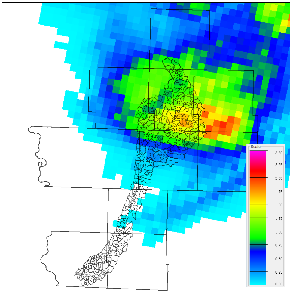
Figure 3.3. Example of the Stage IV rainfall product used as the precipitation input in the East Nishnabotna River Watershed HMS model. The Stage IV product provides hourly cumulative rainfall estimates for each 4 km x 4 km grid cell. The scale shown indicates estimates of the depth of rainfall (in inches) for a one-hour period.
