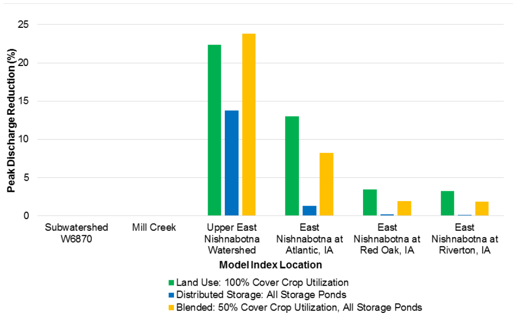
Figure 4.23. Percent reduction in peak discharge at model index locations with implementation of each watershed scenario for the June 2014 event.
