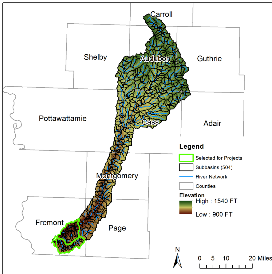
Figure 3.2. HMS model development of the East Nishnabotna River Watershed. We divided the watershed into 504 subbasins for modeling.
