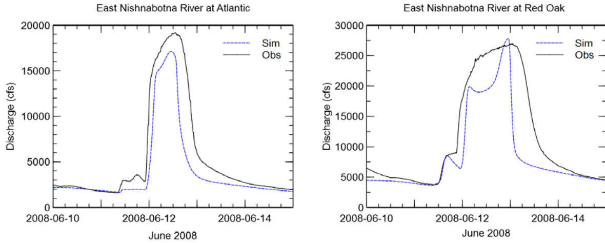
Figure B.7. Validation Storm Events – June 10–15, 2008
