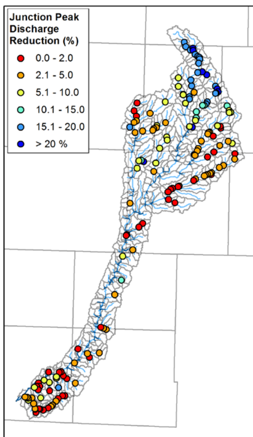
Figure 4.11. Junction peak discharge reductions with ACPF ponds in place for a 6-inch, 24-hour SCS Design Storm. . Simulation results at junctions with large drainage area are not realistic for this design storm event, therefore, results are not shown at junctions with drainage area greater than 100 mi 2 .
