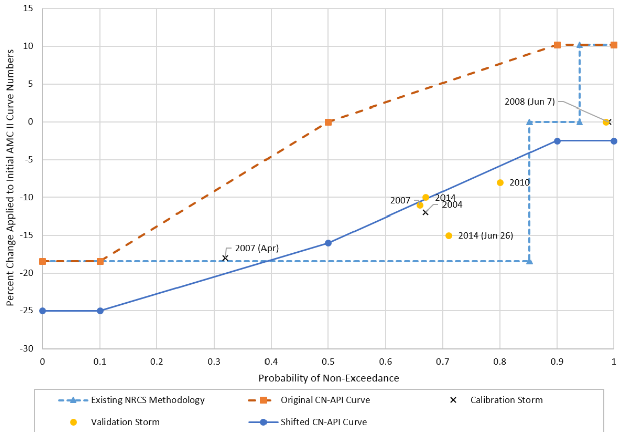
Figure B.2. Accounting for antecedent moisture conditions in the East Nishnabotna HMS model through use of the antecedent precipitation index (API). The researchers used precipitation gauge records to calculate the API prior to each historical storm event and applied a corresponding percent change to each subbasin curve number to account for the initial soil moisture conditions.
