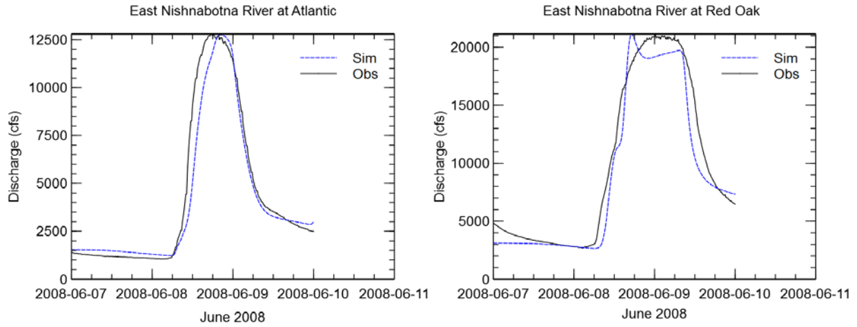
Figure B.5. Calibration Storm Events – June 7–11, 2008
