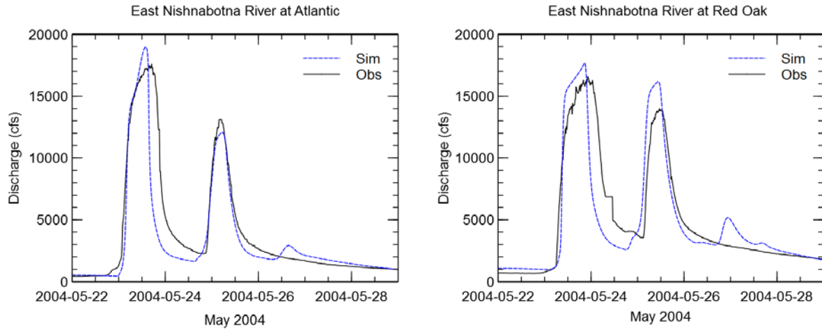
Figure B.3. Calibration Storm Events – May 22–28, 2004
