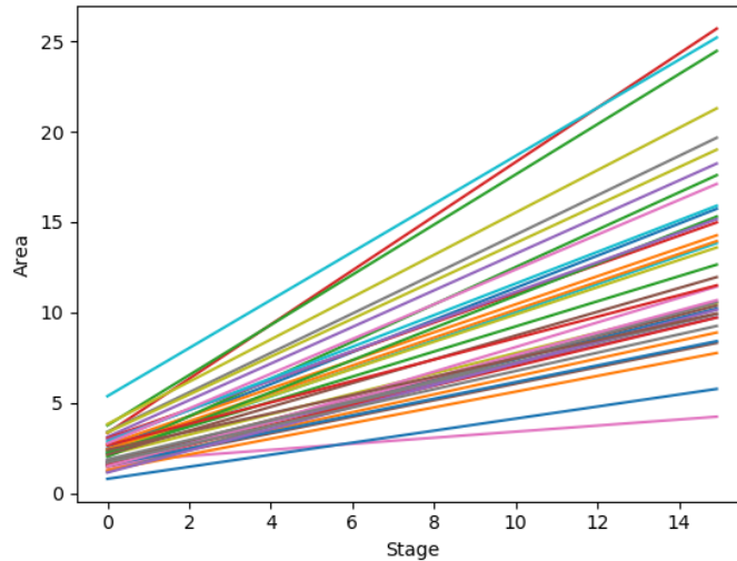
Figure 5.3: Stage-Area Linear Regression for Headwaters North English River NRW. Linear regression stage-area relationship for each site-specific NRW in Headwaters North English River.
