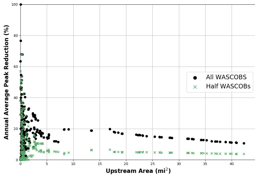
Figure 6.7: Headwaters North English River Peak Reduction with WASC OB Implementation. Average peak reduction in Headwaters North English River for each subbasin downstream of a WASC OB for the two simulations. The first is a full implementation of WASC OBs and the second is a random selection of half the WASC OBs.
