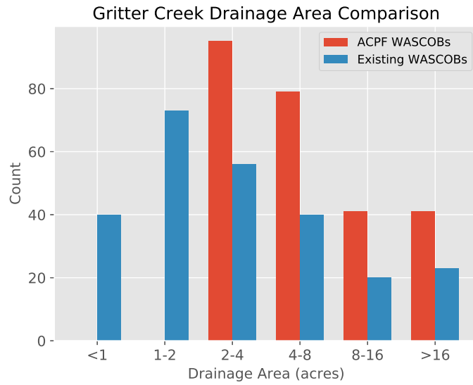
Figure 3.11: Gritter Creek WASCObS Drainage Area Comparison.
