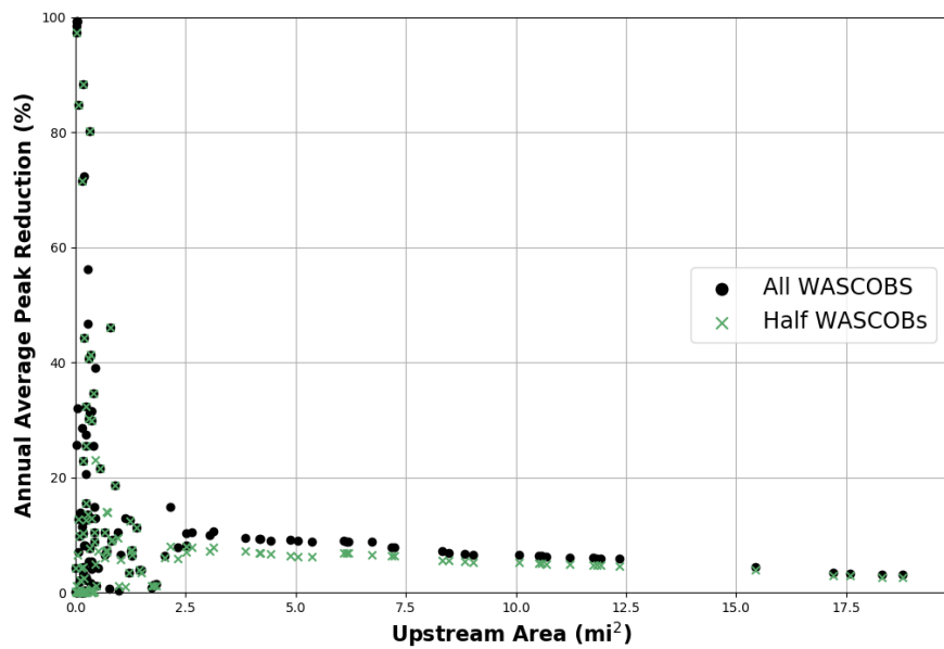
Figure 6.8: Gritter Creek Peak Reduction with WASCORB Implementation. Average peak reduction in Gritter Creek for each subbasin downstream of a WASCORB for the two simulations. The first is a full implementation of WASCORBs and the second is a random selection of half the WASCORBs.
