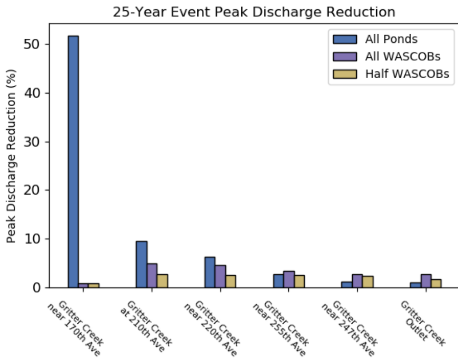
Figure 6.10: 25-Year Event Gritter Creek Peak Reduction. The 25-year return period peak reduction for all scenarios simulated in Gritter Creek.
