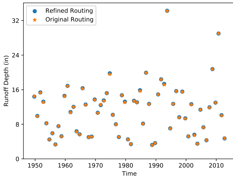
Figure 4.4: Annual Runoff Depth of Original and Refined Headwaters North English River Routing
