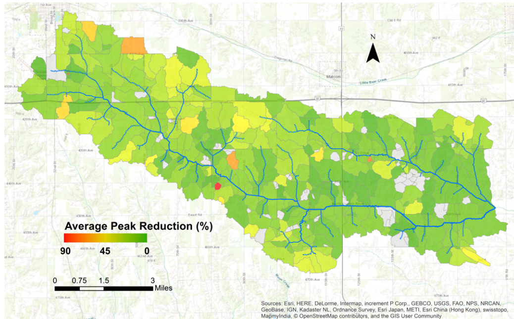
Figure 6.4: Headwaters North English River Peak Reduction with Full WASC OB Implementation. Average peak discharge reduction (in %) for each subbasin in Headwaters North English River between the baseline simulation and the complete WASC OB implementation scenario.
